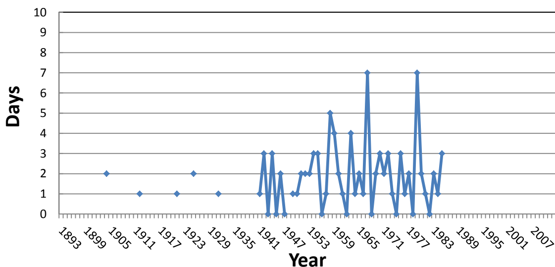
BRDG - Precipitation > 2.0 Inches
