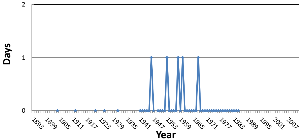
BRDG - Precipitation > 5.0 Inches
