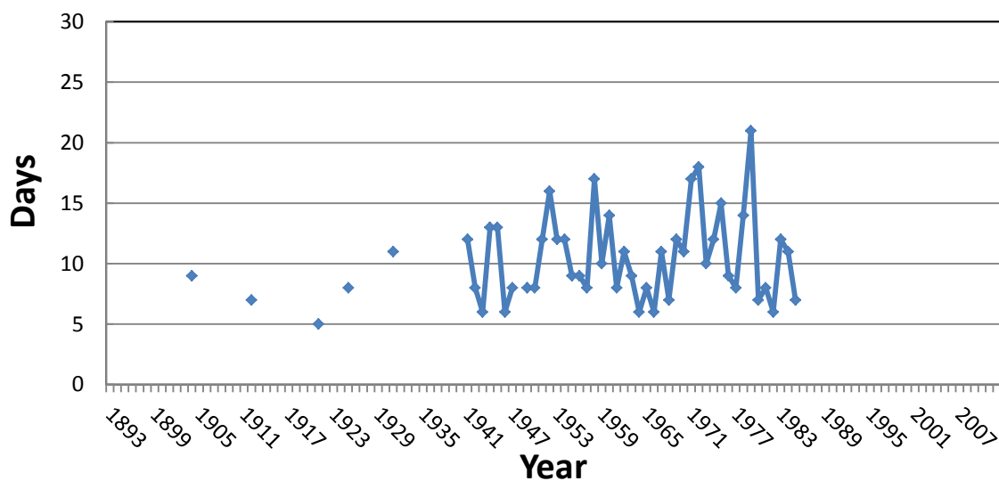
BRDG - Precipitation > 1.0 Inches
