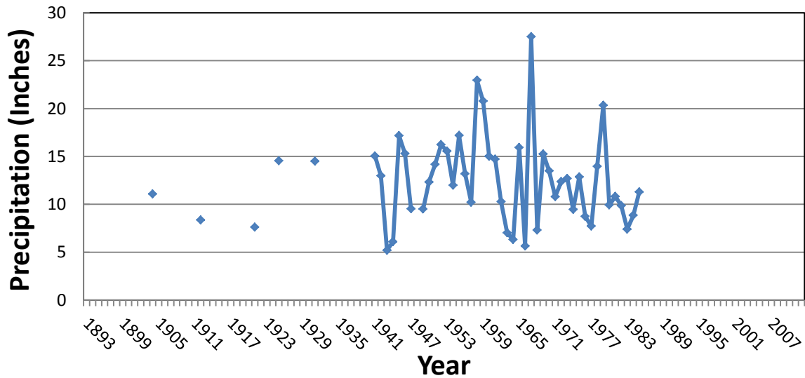
BRDG - Summer Precipitation
