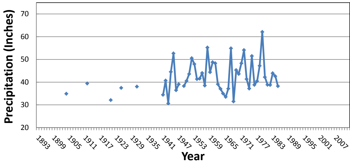
BRDG - Annual Precipitation
