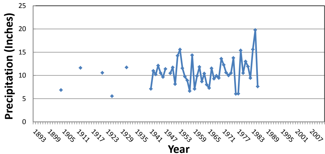
BRDG - Spring Precipitation
